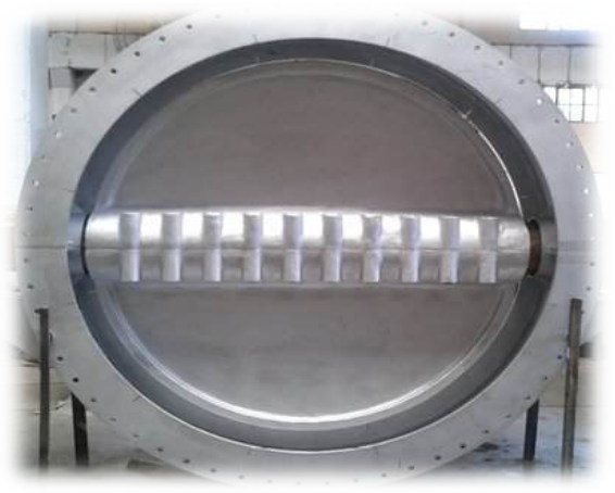
Throttle Flap Valve
