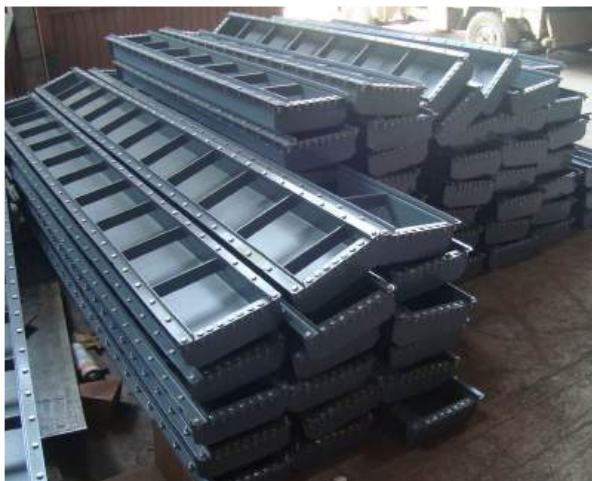
Aeration Trough
