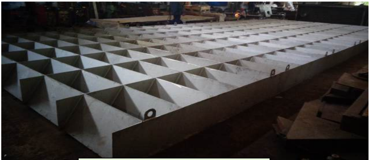
SS Gas Diverting Baffles for Deduster
